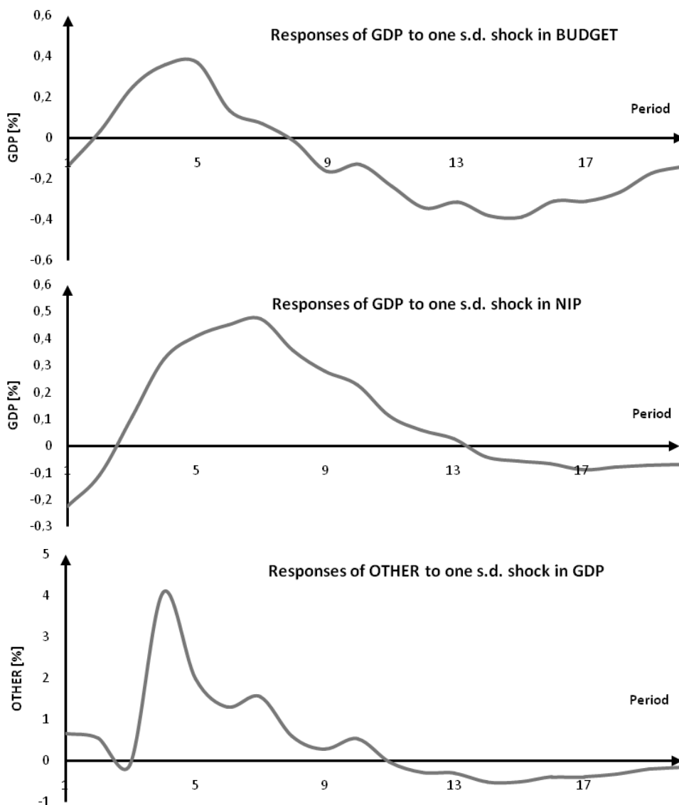
Figure 1. Impulse responses of caused variables to one s.d. shocks in time series of causal factors
